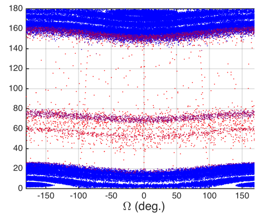
(b) \Omega vs. i for 4 \times 0 shape model
