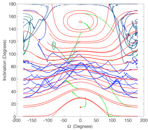
(c) Benu \phi = 15^\circ , 0.477r_L
