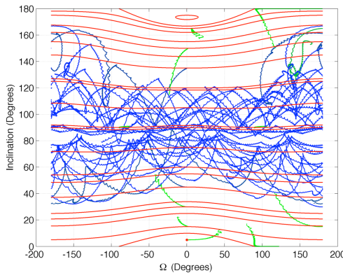
(e) Benu \phi = 25^\circ , 0.673r_L
