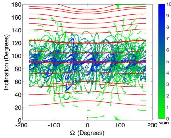
(c) Bennu: b = 100 \text{ kg/m}^2
