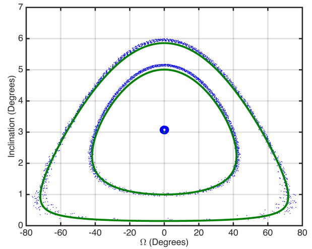
(b) Prograde MLP, D=7.5 m
