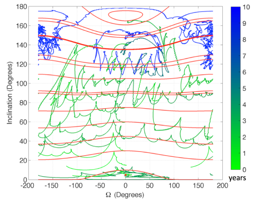
(f) KW4 \phi = 25^\circ , 1.089r_L
