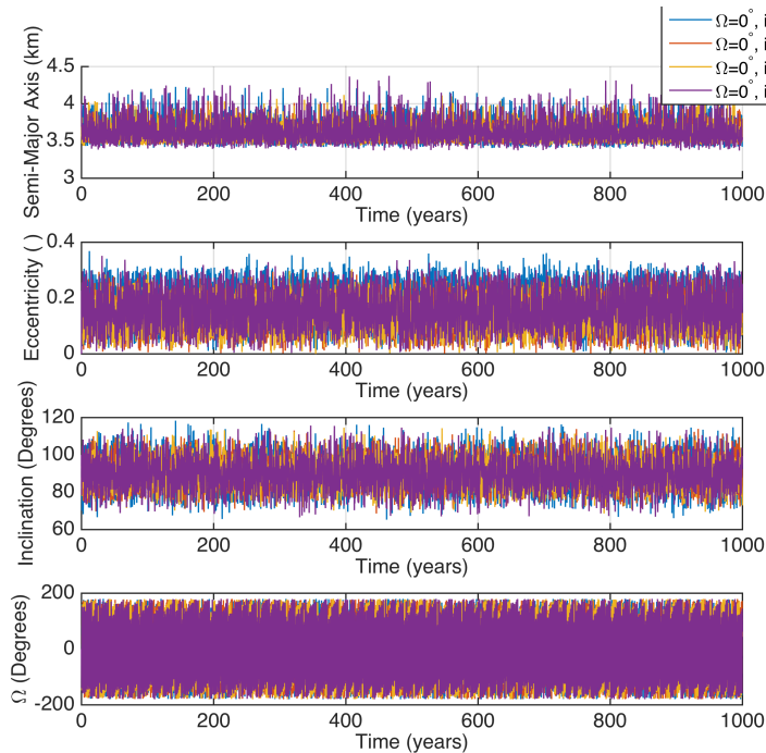
Figure 4.5: Keplerian orbital elements for the 4 stable orbits for a 5.25 cm satellite at 4 km.
