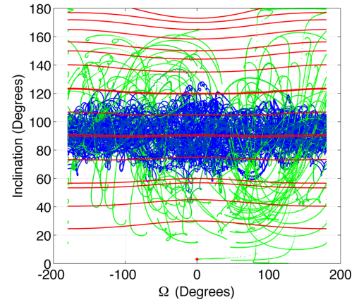
(b) KW 4 : b = 100 \text{ kg/m}^2
