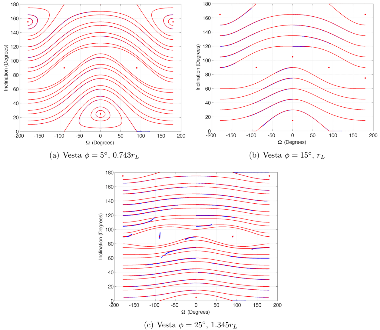
Figure 5.3: These three figures show the numerical results in blue to green and the averaged motion in red. These figures are in the asteroid orbit-frame so the equilibria for the Laplace plane is defined by i = \epsilon - \phi .
