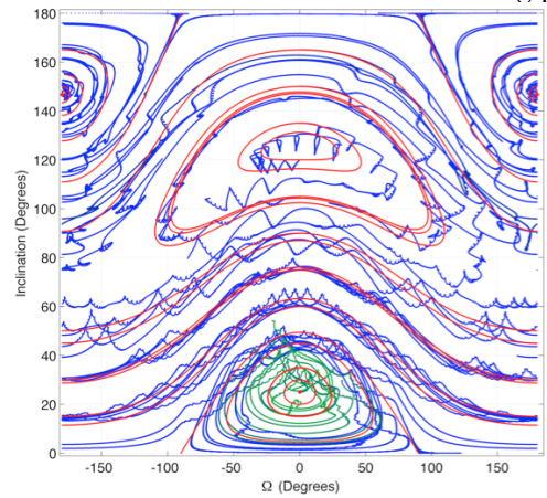
(b) KW4 \phi = 5^\circ , 0.565r_L
