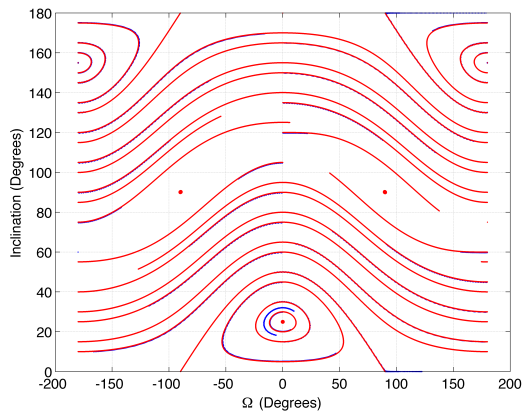
(a) Vesta: b = 100 \text{ kg/m}^2
