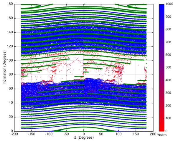
(a) All results
