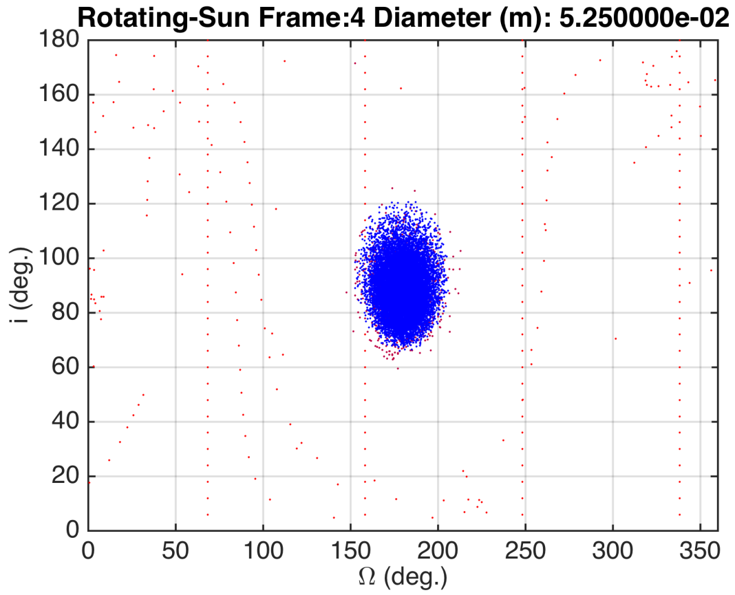
Figure 4.6: Inclination vs. \Omega for 1000 years for i = 84^\circ, 90^\circ, 96^\circ, 102^\circ for a 5.25 cm satellite at 4 km.
