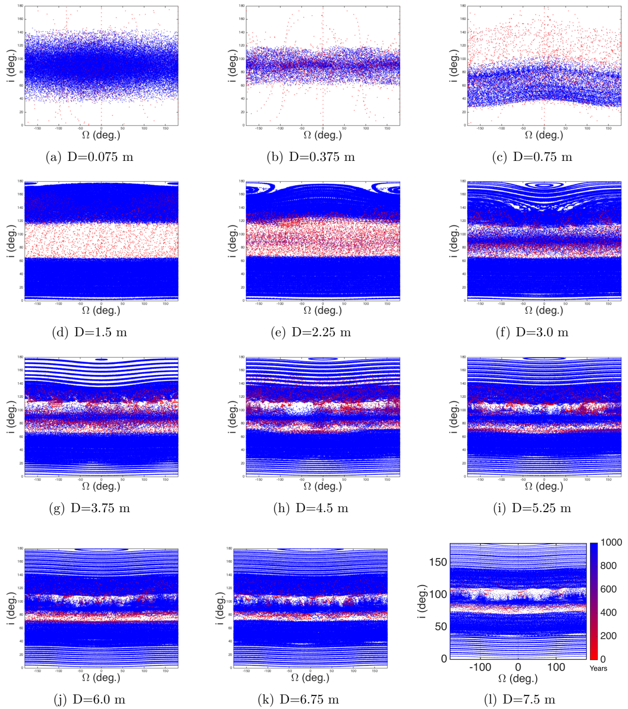
Figure 4.4: Evolution of the orbital planes at a semi-major axis of 4 km for various satellite diameters.
