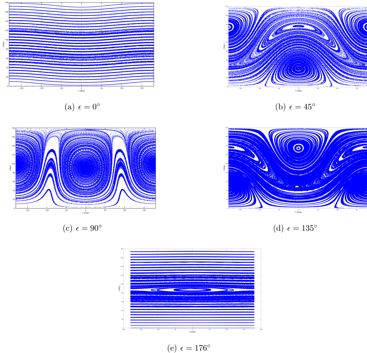
Figure 5.16: Inclination vs. longitude of the ascending node for a = 2 \text{ km} , D = 3.75 \text{ m} for 1000 years. The higher obliquity asteroids, have the motion of the natural satellite orbits oscillating around the Laplace plane, and therefore their longitude of the ascending node is bounded. Figure (a), has a small retrograde obliquity, therefore the longitude of the ascending node is not bounded to the Laplace plane.
