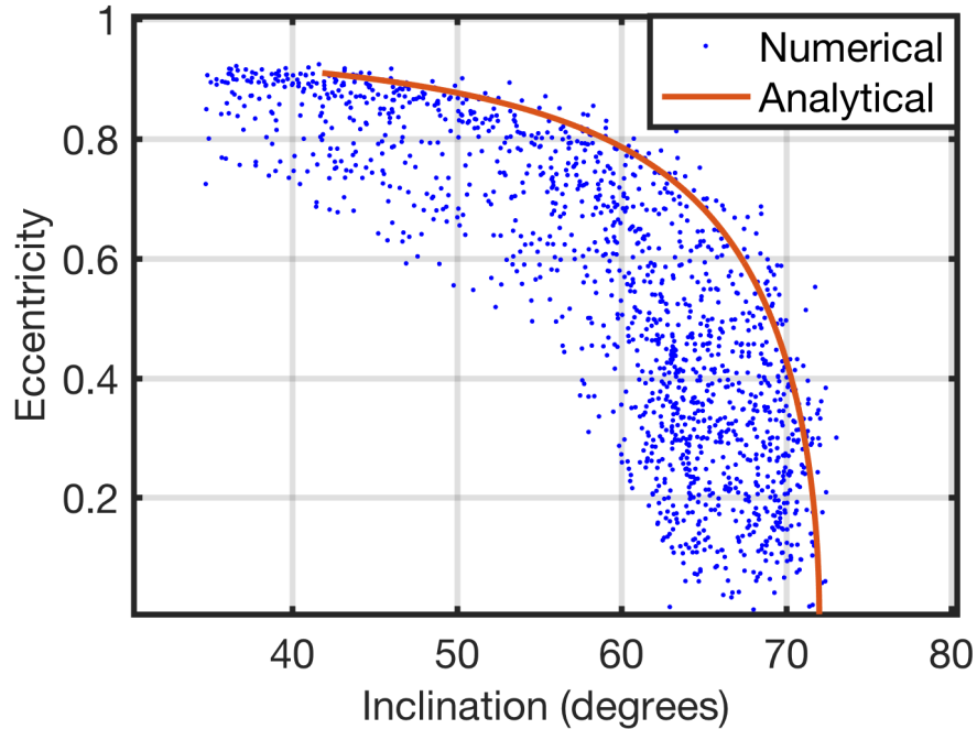
Figure 4.9: The numerical and analytical data for the Kozai resonance at a = 10 \text{ km} , D = 7.5 \text{ m} , \Omega = 0^\circ , i = 72^\circ .
