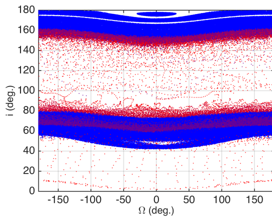
(a) \Omega vs. i for J_2 shape model
