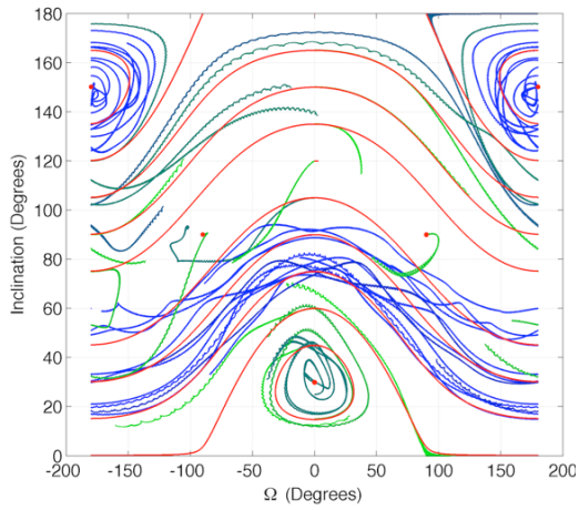
(a) Benu \phi = 5^\circ , 0.337r_L
