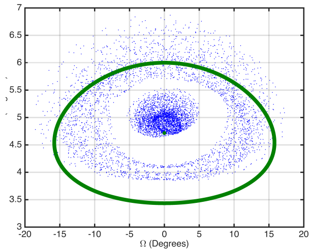
(c) Prograde MLP, D=1.5 m
