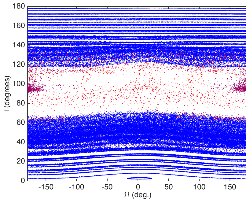
Figure 4.10: Inclination vs. \Omega for a = 4 \text{ km} , D = 5.25 \text{ m} for 10,000 years.
