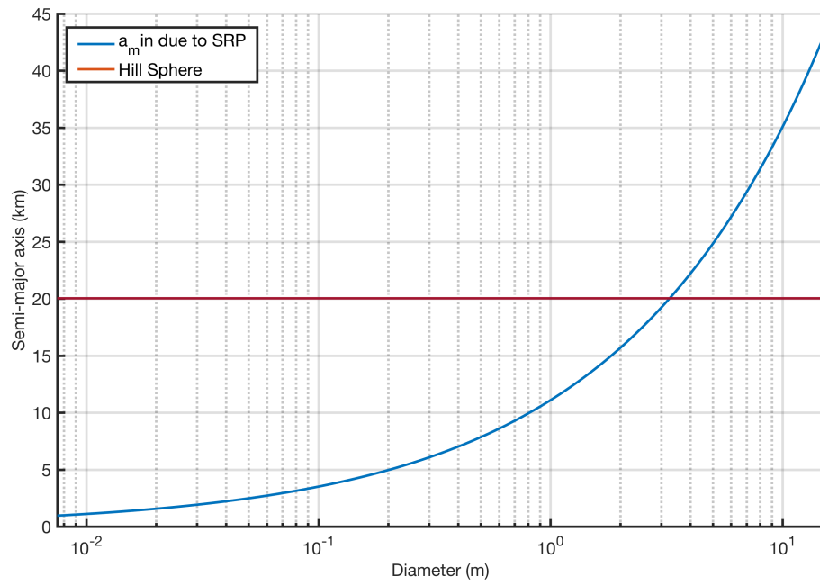
Figure 4.1: The Hill sphere and SRP no-escape criteria for Benu.
