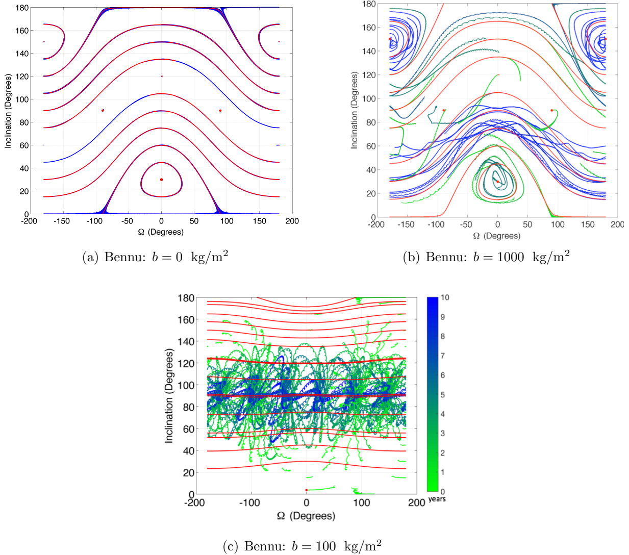
Figure 5.5: These three figures show the numerical results in blue to green and the averaged motion in red. The trajectories go from green to blue, depending how long the trajectory exists without escape or collision. The colormap on the right gives the time in years that corresponds to a given color. Each plot was evaluated at Benu at \epsilon = 30^\circ and a = 0.337r_L \approx 3 \text{ km} . These figures are in the asteroid orbit frame so the equilibria for the Laplace plane is defined by i = \epsilon - \phi .
