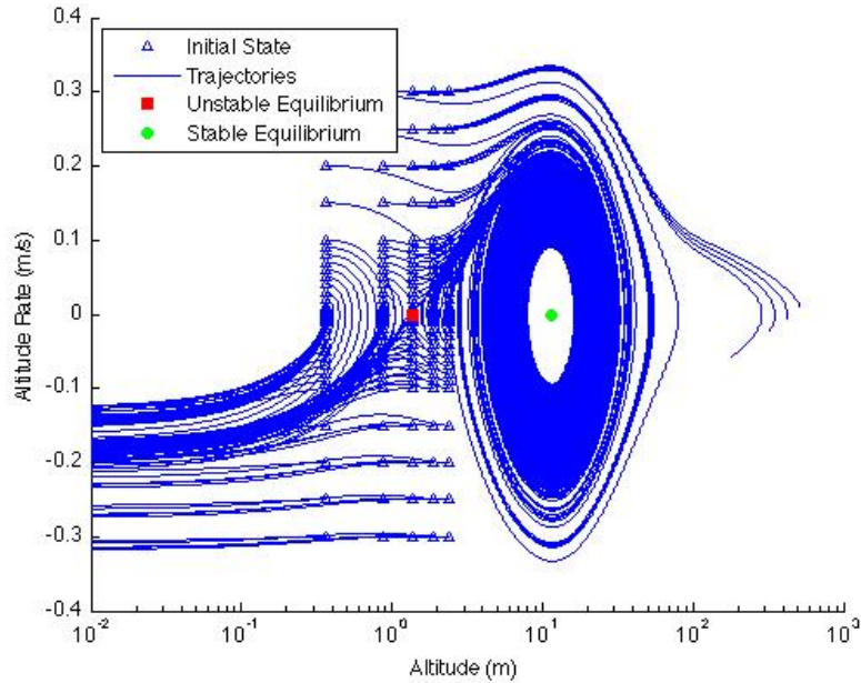
Figure 5.15: Altitude and altitude rate for a 0.57224 micron radius particle near Itokawa using the numerically-described non-monotonic sheath.
