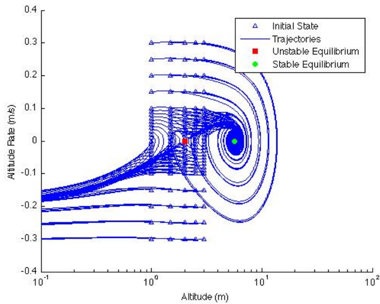
Figure 5.12: Altitude and altitude rate for a 0.57224 micron radius particle near Eros using the numerically-described non-monotonic sheath.
