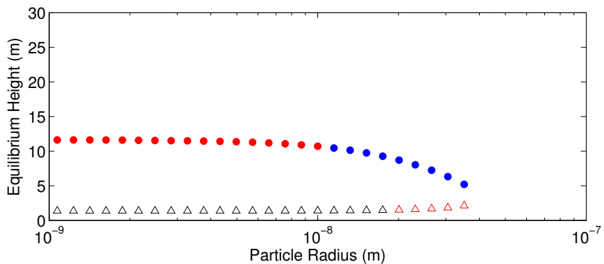
(a) Moon
