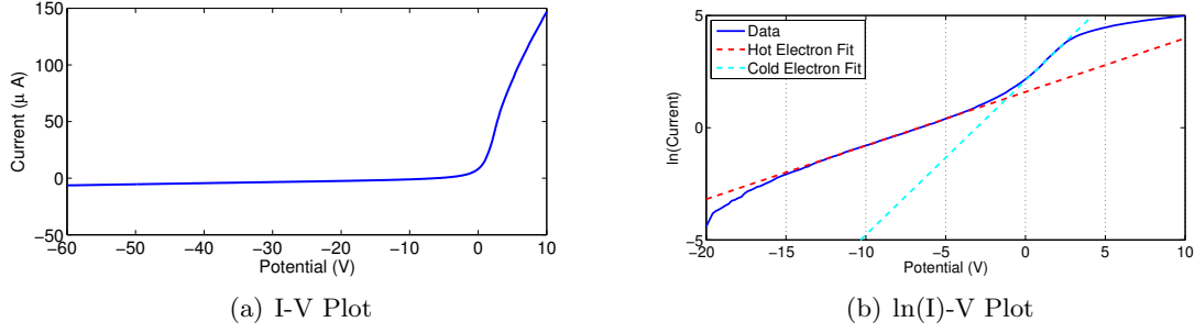
Figure 4.8: Current vs potential plot measured with a Langmuir probe to determine the characteristics of the plasma. In (b), the ion current has been removed. Plasma Potential: 2.6V.
