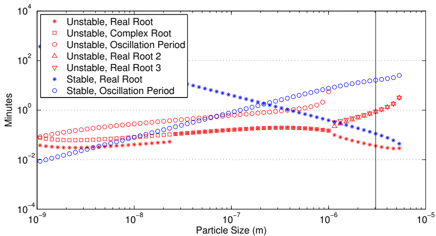
(a) Itokawa
