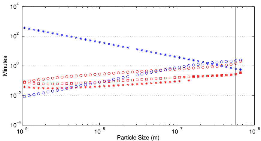
(b) Eros
