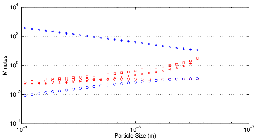
(c) Moon
