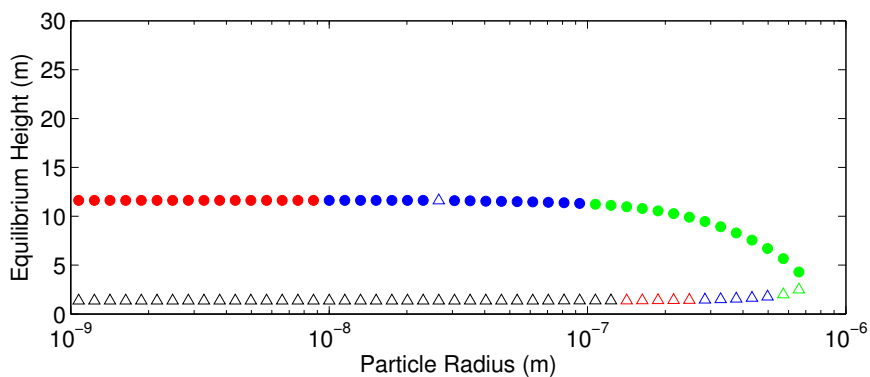
(b) Eros
