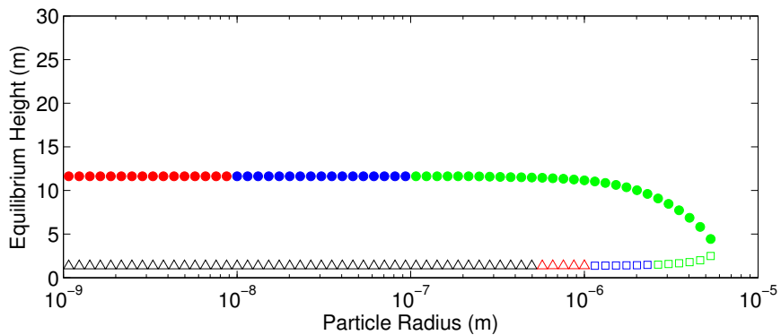
(c) Itokawa
