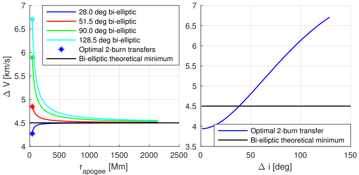
Figure 2.4: Comparison between a two- and a three-burn strategy. Left: \Delta V in function of r_{\text{apogee}} . Right: \Delta V in function of total required \Delta i .
