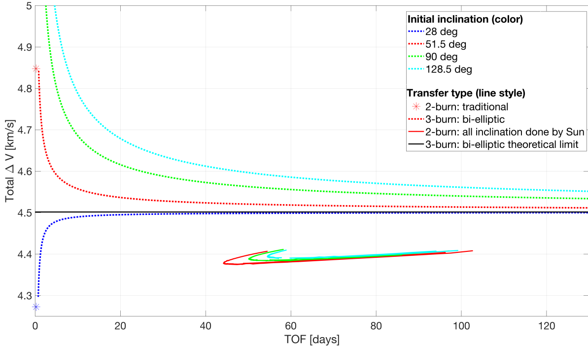
Figure 3.11: \Delta V and TOF comparison for different transfer strategies from inclined LEO to GEO.
