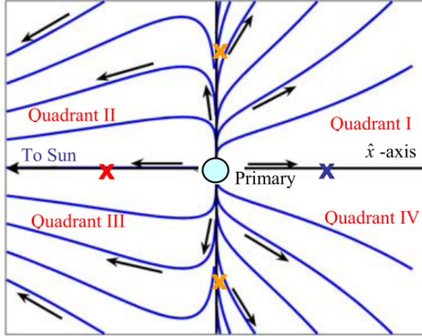
Figure 2.14: Visualization of the solar tidal accelerations in the Sun-Saturn system, in function of the quadrants defined in the rotating frame. The effects are exaggerated by introducing an artificially large primary and magnifying the \hat{y} -components (credit: Davis [60]).
