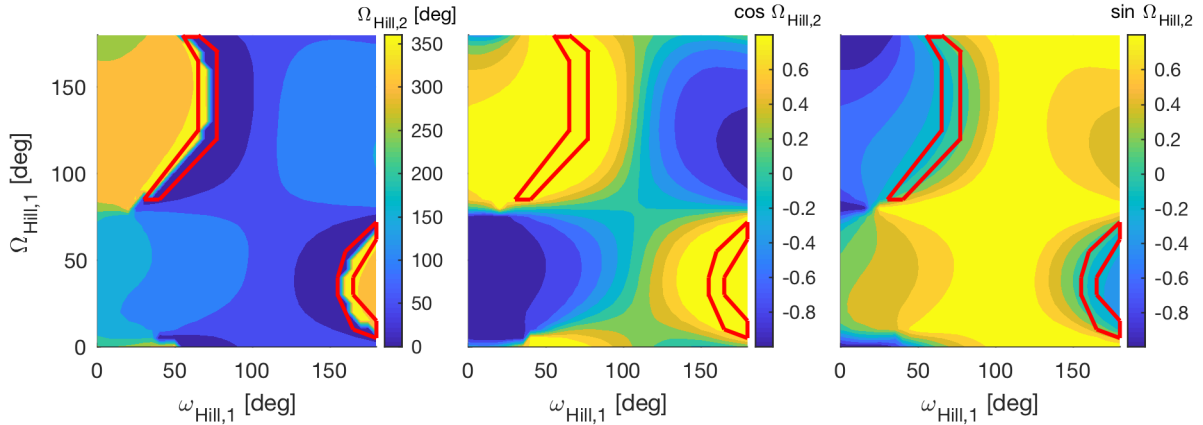
Figure 5.1: Example of how an artificial angular bifurcation can be resolved by splitting the angle in its cosine and sine components. In the regions indicated in red, the angle passes through the 360^\circ - 0^\circ region, introducing strong gradients on the contours. Those are not present in the cosine and sine components.
