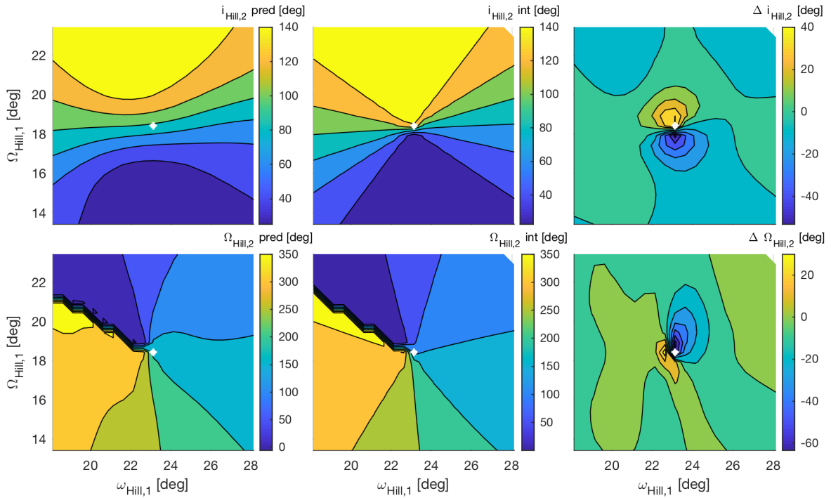
Figure 5.8: Comparison between the predicted and integrated response in the neighborhood of a point from the Monte Carlo analysis with a large error in i_{\text{Hill},2} and \Omega_{\text{Hill},2} (white asterisk).
