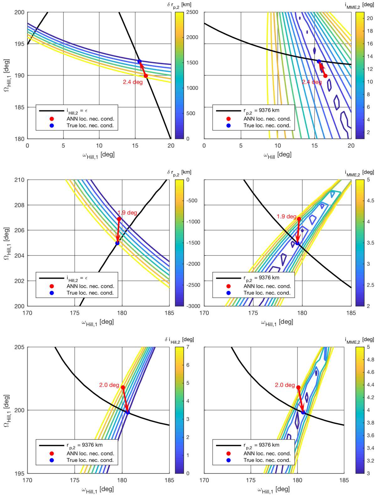
Figure 5.14: Visualization of the deviations from the locations of the necessary conditions predicted using the scaled Hill ANN, and their true location and the effect on i_{MME,2} when integrated in the eccentric Hill system, for transfers 1 (top), 2 (middle), and 3 (bottom).
