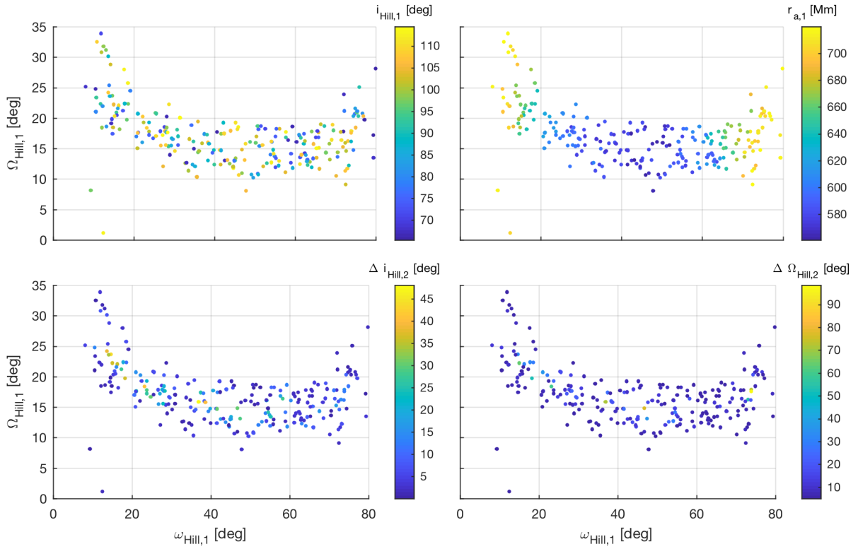
Figure 5.7: Region in initial orbital elements-space where the errors in i_{\text{Hill},2} or \Omega_{\text{Hill},2} are larger than 5^\circ for the 100,000 samples in the Monte Carlo analysis for the circular Hill system.
