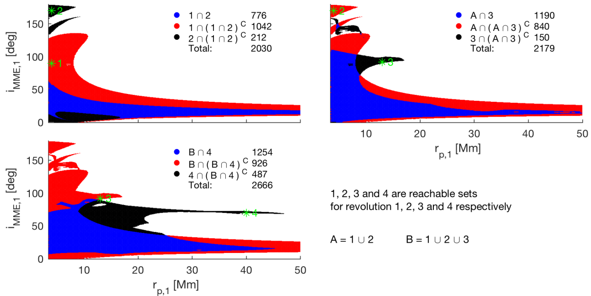
Figure 6.3: Visualization of the effect of additional loops on the r_{p,1} - i_{\text{MME},1} plane for ballistic transfers arriving at Phobos at day 0. Loop 2, 3, and 4, add 212, 150 and 487 [Mm \times deg], respectively. One transfer per loop (green) is selected to be discussed in more detail.
