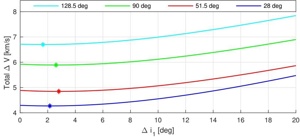
Figure 2.3: Determine initial inclination change to minimize total fuel cost for a two-burn strategy. The different colors indicate different total inclination changes, the asterisks the optimum initial inclination changes to minimize the total fuel cost.
