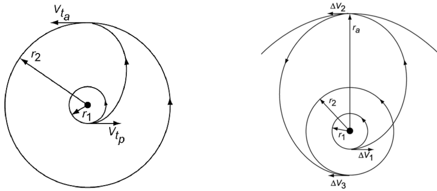
Figure 2.2: Visualization of a Hohmann and a bi-elliptic co-planar transfer (credit Wakker [43]).
