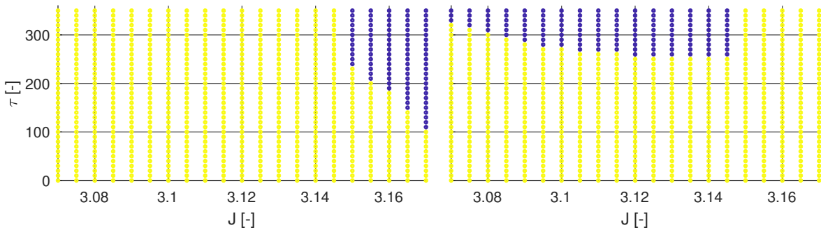
Figure 5.55: Classification whether or not a periaapse on the stable manifolds of L_2 exists for group 1 (left) and 2 (right): periaapse exists (yellow) or periaapse does not exist (blue).
