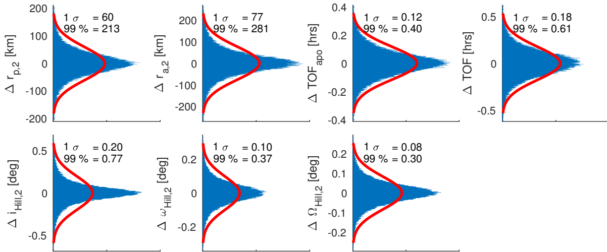
Figure 5.20: Distribution of the errors between the predicted and integrated apoareion scaled circular Hill Poincaré map for the 100,000 sampled points in the Monte Carlo simulation, excluding the grey buffer regions. The x-axis shows the number of samples for each y-axis bin.
