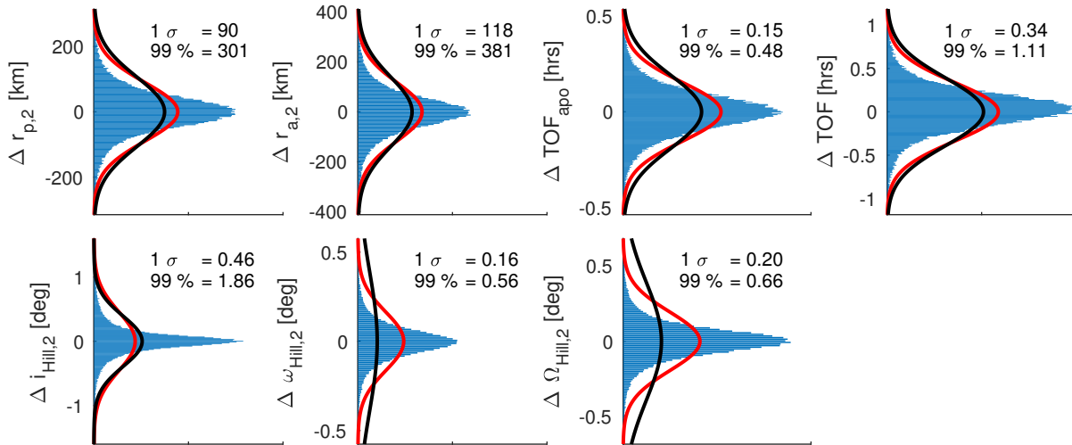
Figure 5.28: Distribution of the errors of the predicted orbital elements at periareion two using the entire architecture, compared to the orbital elements integrated in the eccentric Hill system for the 100,000 sample points in the Monte Carlo simulation of the entire architecture. The x-axis shows the number of samples for each y-axis bin.
