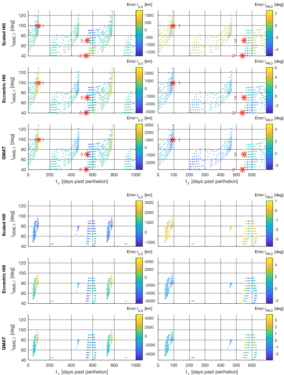
Figure 5.13: Error breakdown of the transfers predicted to arrive at Phobos' (top) and Deimos' (bottom) r_p and i_{MME} at periareion two in the apoareion scaled circular Hill dynamical systems. Top: error in arrival conditions when integrating the predicted initial states in the apoareion scaled Hill system. Middle: errors integrated in the eccentric Hill system. Bottom: errors integrated in the DE405 ephemeris in GMAT.
