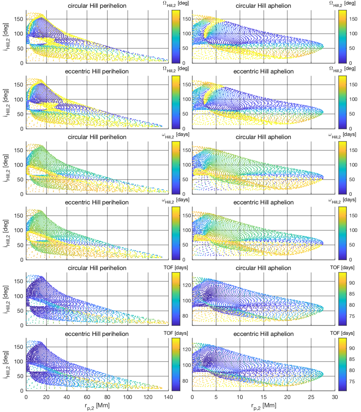
Figure 4.10: Comparison between the response of the second periareion for initial orbital elements e_1 = 0.99 and i_{\text{Hill},1} = 65^\circ integrated to the next periareion in the scaled circular Hill approximation and eccentric Hill system: \Omega_{\text{Hill},2} (top), \omega_{\text{Hill},2} (middle) and TOF (bottom) when Mars is at perihelion (left) and aphelion (right).
