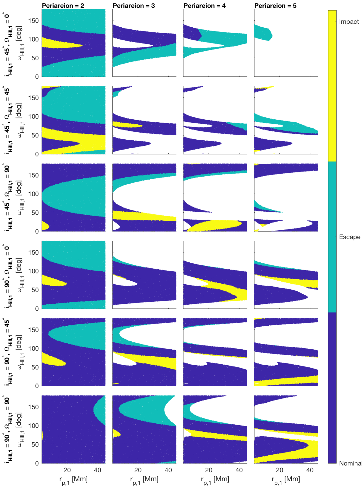
Figure 6.41: Impact and escape characteristics for the next four periareions for multiple combinations of i_{\text{Hill},1} and \Omega_{\text{Hill},1} with r_{a,1} = 700,000 km, departing when Mars is at perihelion.
