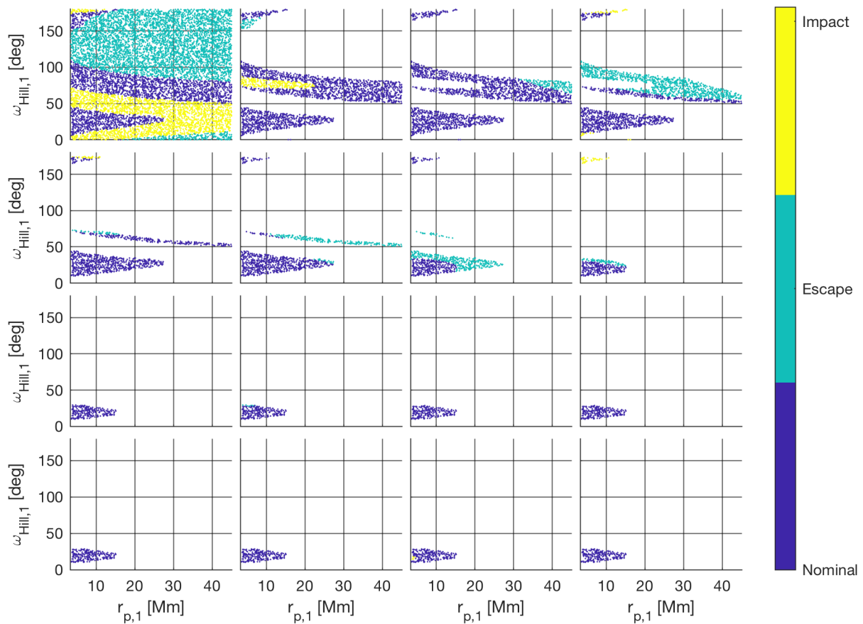
Figure 6.43: Impact and escape characteristics for next 16 periareions for i_{\text{Hill},1} = 45^\circ , \Omega_{\text{Hill},1} = 45^\circ with r_{a,1} = 700,000 km, departing when Mars is at perihelion.
