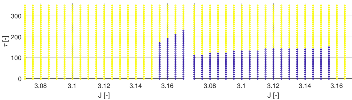
Figure 5.53: Classification whether or not a periaapse on the unstable manifolds of L_1 exists for group 1 (left) and 2 (right): periaapse exists (yellow) or periaapse does not exist (blue).
