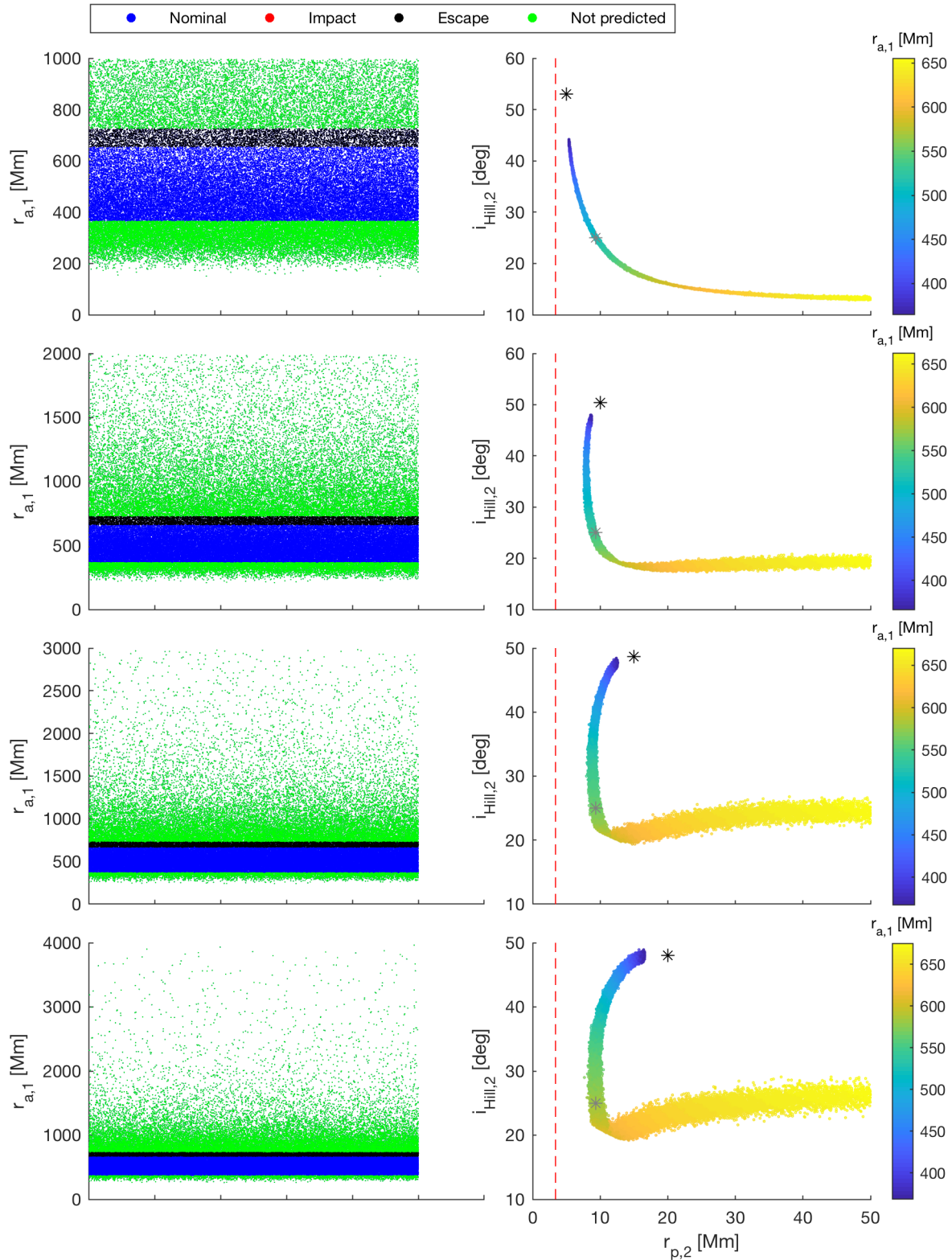
Figure 6.36: Results of the Monte Carlo injection error analysis for group 2 with constant i_{\text{MME},1} . From top to bottom: trajectory 5 through 8. Left: perturbed r_{a,1} and classifications for the next predicted periareion. Right: r_{p,2} and i_{\text{Hill},2} at the next periareion, in function of original r_{a,1} . Red dashed line represents the Martian surface.
