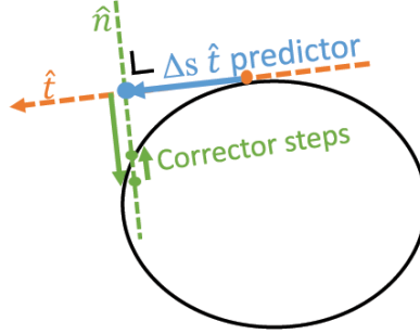
Figure 3.4: Visualization of the pseudo-arclength constraint.
