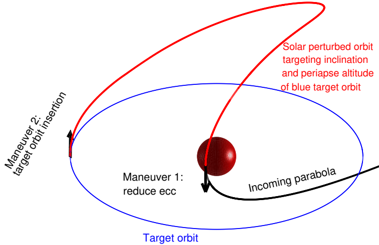
Figure 4.2: Schematic of the solar gravity driven transfer structure around Mars. Not to scale: red solar perturbed orbit has an apoapse radius \mathcal{O}(10^5 \text{ km}) , blue target orbit has a radius \mathcal{O}(10^3\text{-}10^4 \text{ km}) .
