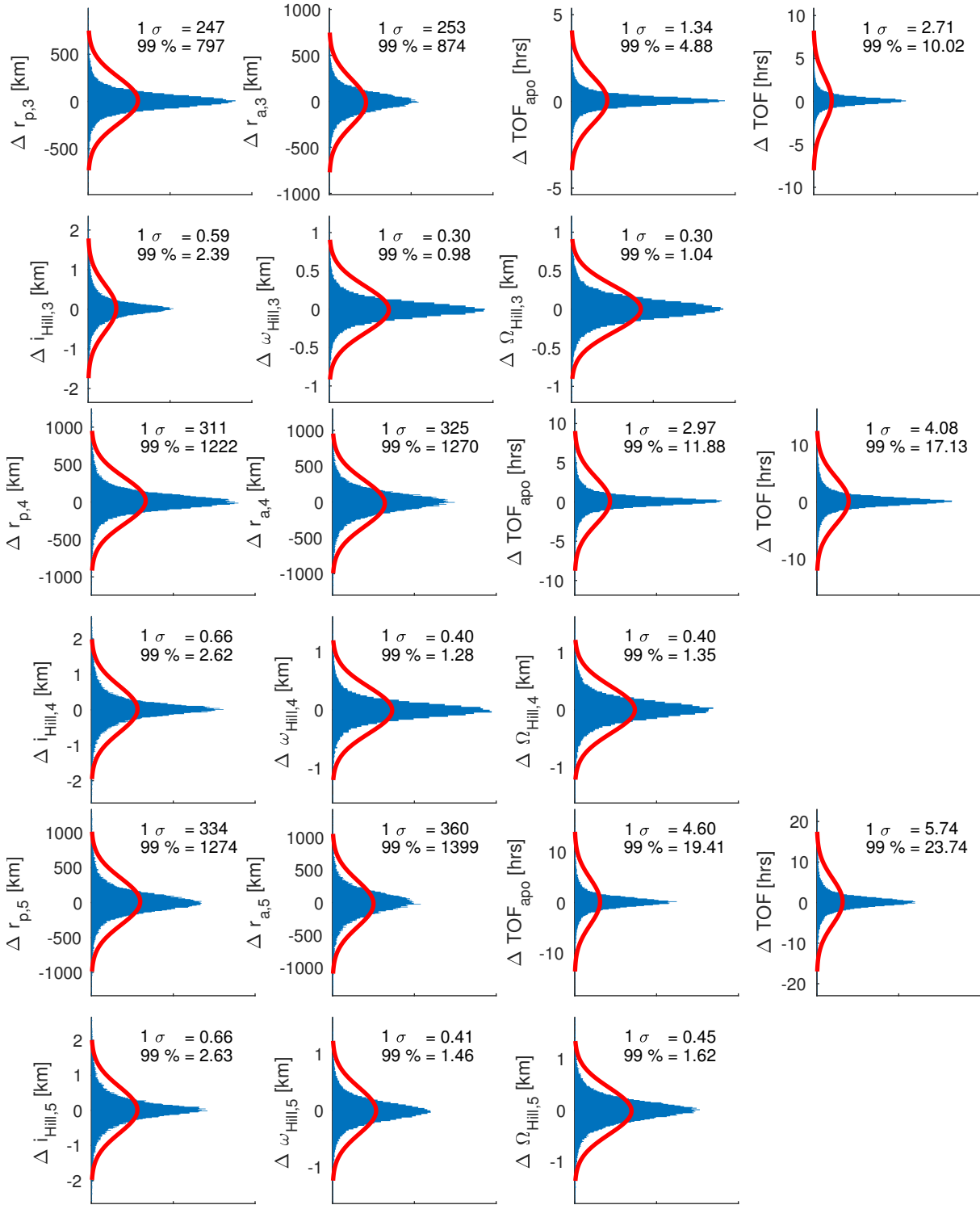
Figure 5.31: Distribution of the errors of the predicted orbital elements at periareons three, four, and five, using the entire architecture, compared to the orbital elements integrated in the eccentric Hill system for the 10,000 sample points in the Monte Carlo simulation of the entire architecture. The x-axis shows the number of samples for each y-axis bin.
