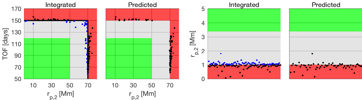
Figure 5.26: Comparison of the integrated versus predicted results for erroneously classified transfers: false positives (blue), false negatives (black), for escape (left) and impact (right) classification.
