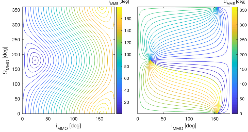
Figure 2.12: Coupling between i and \Omega for the equatorial and ecliptic reference frame. As an example, the MME and MMO frames are shown, centered around Mars with angular difference \epsilon = 25.19^\circ .
