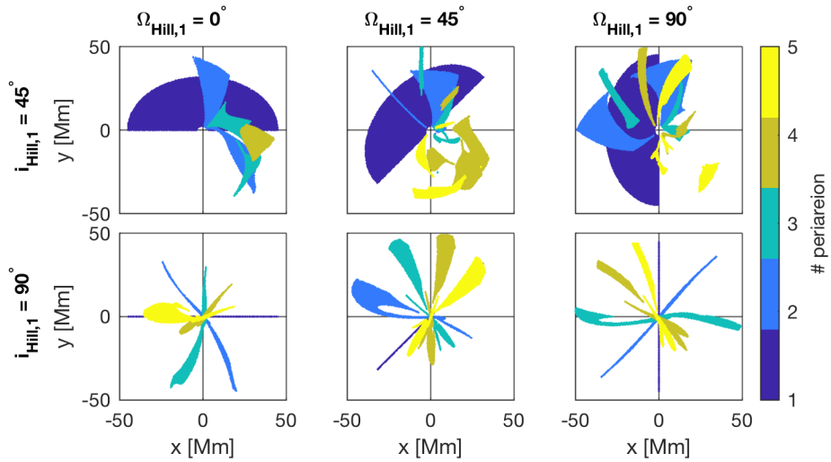
Figure 6.42: xy projection of periareions 1 through 5 for multiple combinations of i_{\text{Hill},1} and \Omega_{\text{Hill},1} with r_{a,1} = 700,000 km, departing when Mars is at perihelion.
