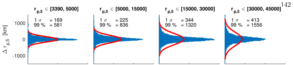
Figure 5.32: Distribution statistics of the errors of the predicted orbital elements at the fifth periastron using the ANN architecture for multiple loops, compared to the orbital elements integrated in the eccentric Hill system for different orbital regimes of r_{p,5} . The x-axis shows the number of samples for each y-axis bin.
