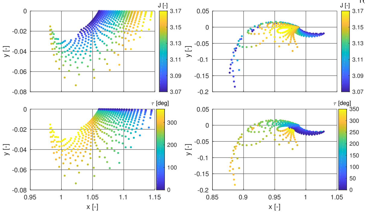
Figure 5.54: Periaapse group identification on the stable manifolds of L_2 : group 1 (left) and 2 (right).
