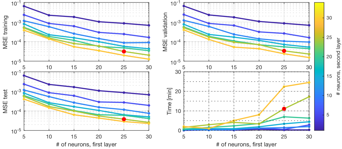
Figure 5.4: Hidden layers and neurons architecture trade-off for i_{\text{Hill},2} . The MSE for the training, validation and test set are shown, along with the training time for different number of neurons and different number of layers.
